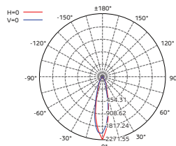
Lux Distance Curve
